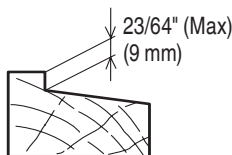
Fig. 2-D (Tapering)
