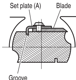
Fig. 10 (Correct installation)
