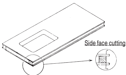
Fig. 2-E (Side planing of flush door)
