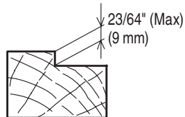
Fig. 2-C (Rabbeting)
